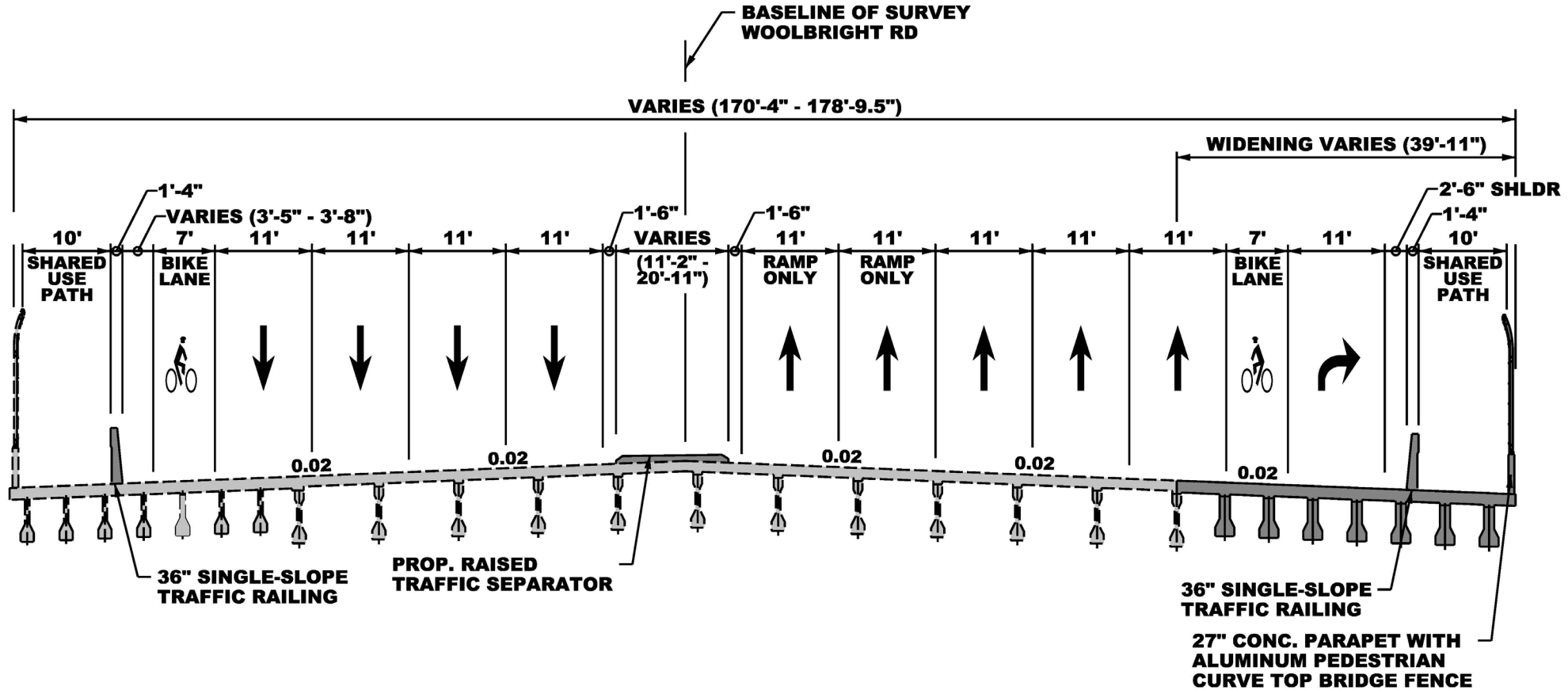
Bridge over SFRC/CSX Railroad
