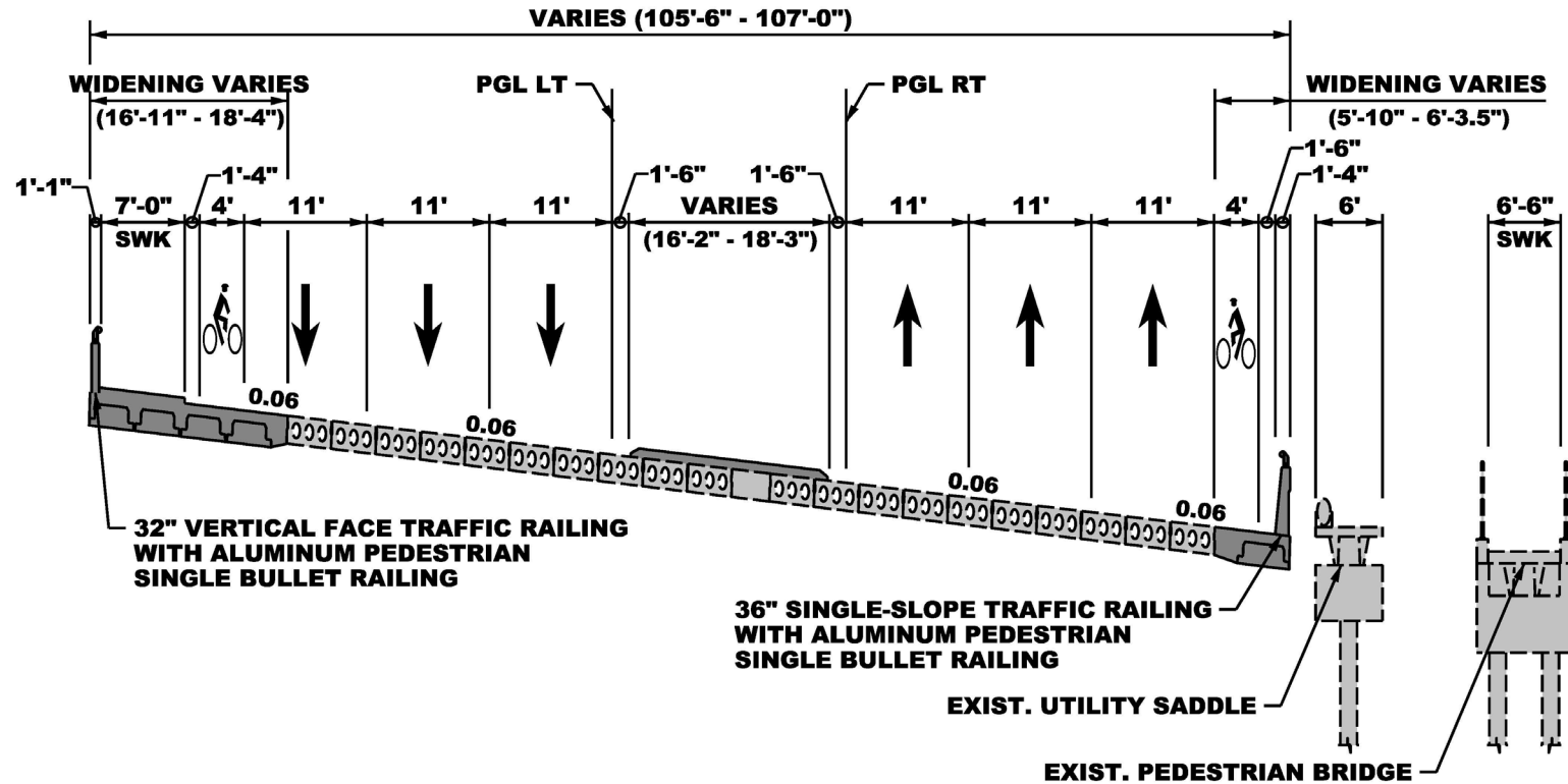
Bridge over LWDD E-4 Canal
